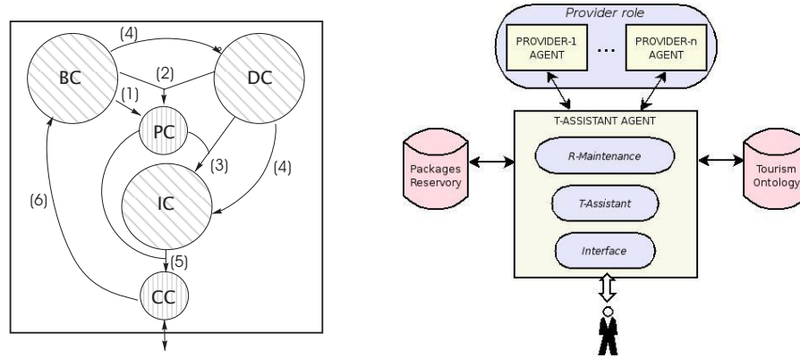
Fig. 1. Multi-context model of a graded BDI agent (left) and the multiagent architecture of the Tourism Recommender system (right)
