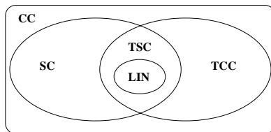
Figure 5: Hierarchy of consistency models
